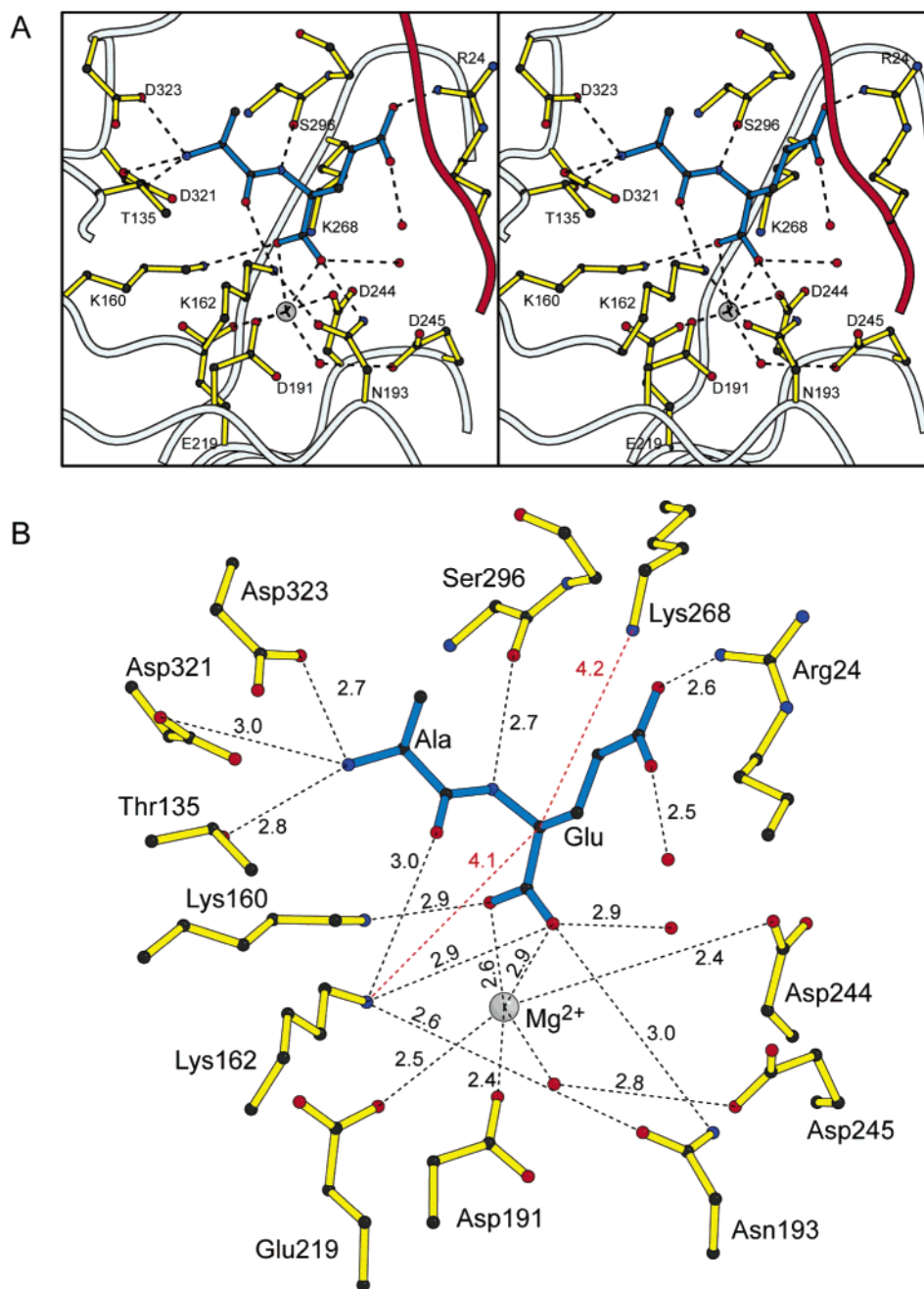
FIGURE 3: Ligand interactions between L-Ala-D/L-Glu and the AE epimerase from B. subtilis . (A) Stereo representation of the important polar interactions between L-Ala-D/L-Glu and the active site. (B) Expanded schematic view of the active site revealing the lengths (in angstroms) of the polar contacts between the substrate and metal ion. This figure was prepared with Bobscript (28).
